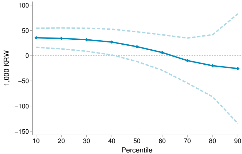
Figure 7: Quantile treatment effect estimates on expenditure.
